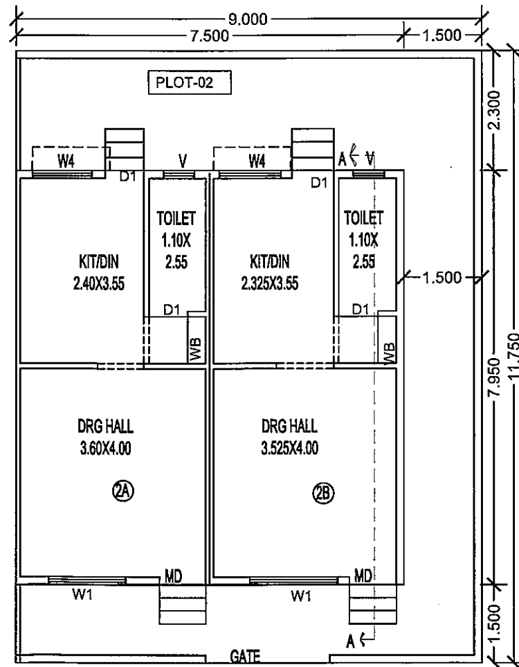
GROUND FLOOR PLAN (2)
