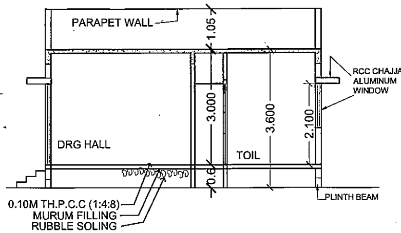
TYPICAL SECTION (2)
