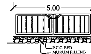
MAIN GATE SECTION
