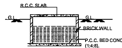
SECTION AT C-C U.G. WATER TANK
