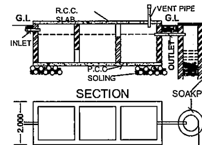
PLAN TYPICAL SEPTIC TANK & SOAK PIT DETAILS
