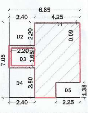
BASEMENT FLOOR BLOCK PLAN ( RESI.) A2 - BUILDING
