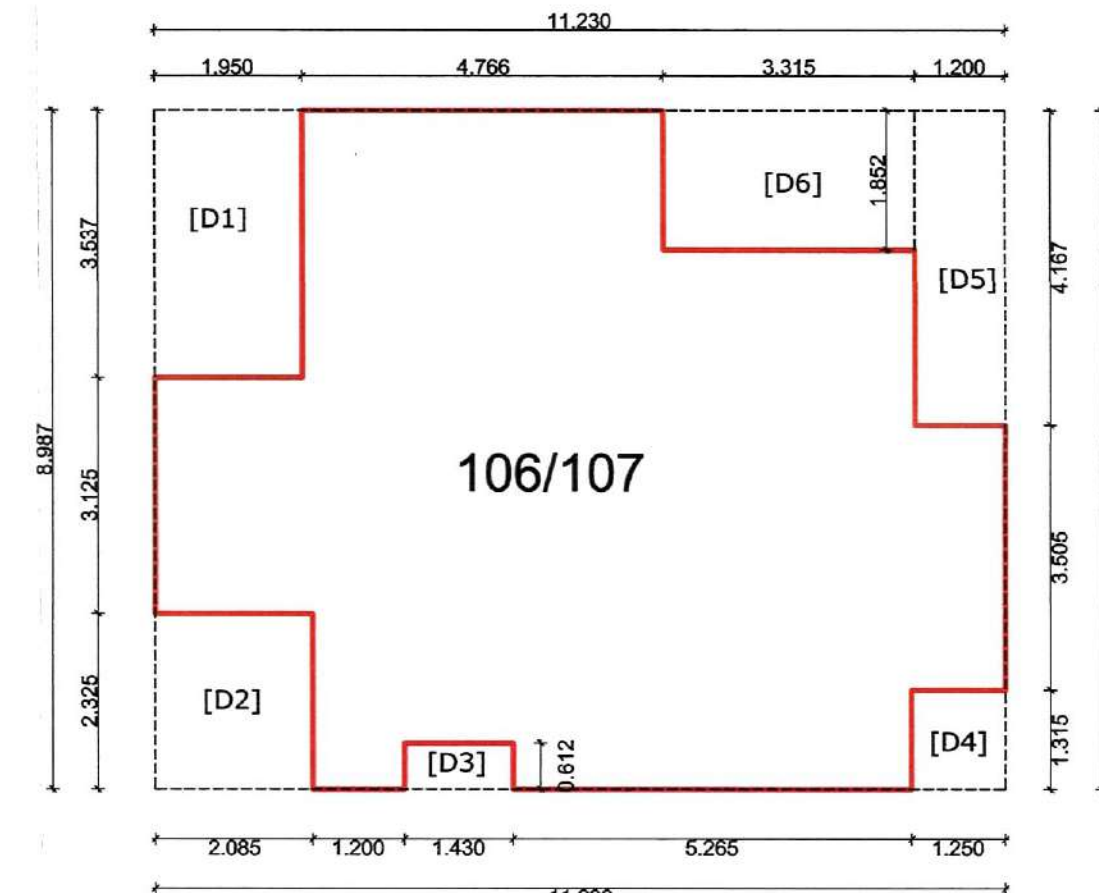
TOWER B:- 3 BHK CARPET AREA BLOCK DIAGRAM FLAT NO. 106,107,206,207,306,307,406,407,506,507,606,607,706,707, 806,906,907,1006,1007,1106,1107,1206,1207,1306,1307
