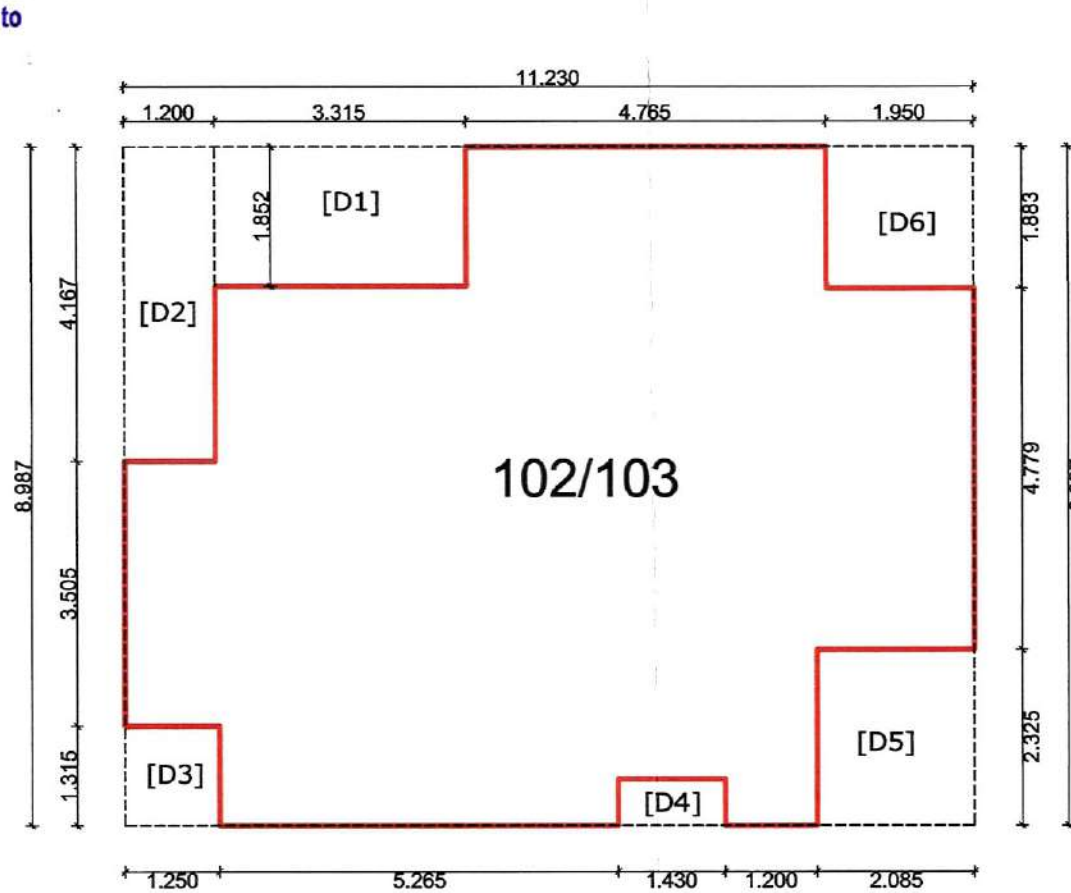
TOWER B:- 3 BHK CARPET AREA BLOCK DIAGRAM FLAT NO. 102,103,202,203,302,303,402,403,502,503,602,603,702, 703,803,903,903,1002,1003,1102,1103,1202,1203,1303,
