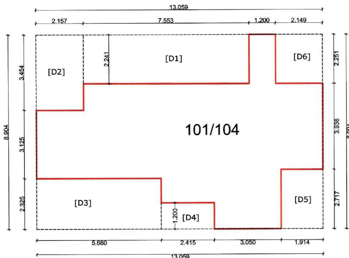
TOWER B:- 3 BHK CARPET AREA BLOCK DIAGRAM FLAT NO. 101,104,201,204,301,304,401,404,501,504,601,604, 701,704,804,901,904,1001,1004,1101,1104,1201,1204,1304,
