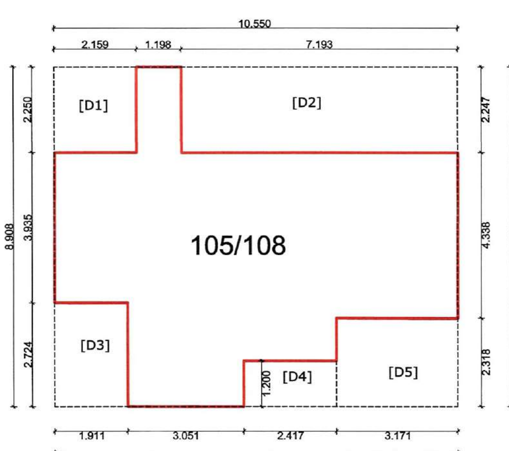
TOWER B:- 3 BHK CARPET AREA BLOCK DIAGRAM FLAT NO. 105,108,205,208,305,308,405,408,505,508,605,608,705, 708,805,905,908,1005,1008,1105,1108,1205,1208,1305,
