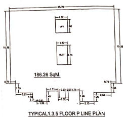
TYPICAL 1,3,5 FLOOR P LINE PLAN
