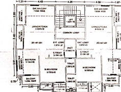
TYPICAL 2.4.6 FLOOR PLAN
