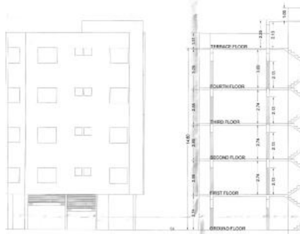
ONT ELEVATION SCALE 1:100 SECTION AA' SCALE 1:100
