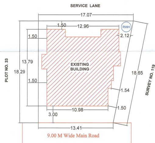
SITE PLAN
