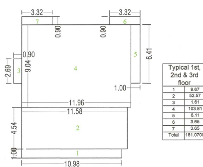
TYPICAL - 1, 2, 3 FLOOR AREA
