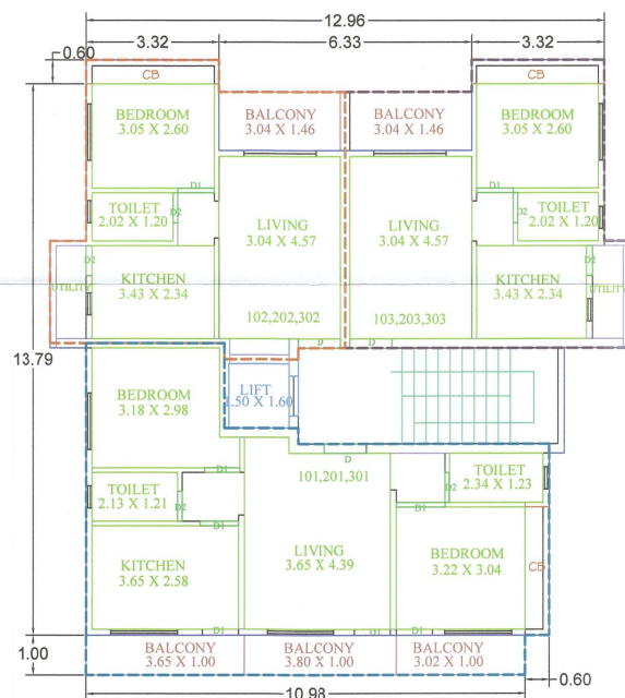
TYPICAL 1st, 2nd & 3rd FLOOR PLAN
