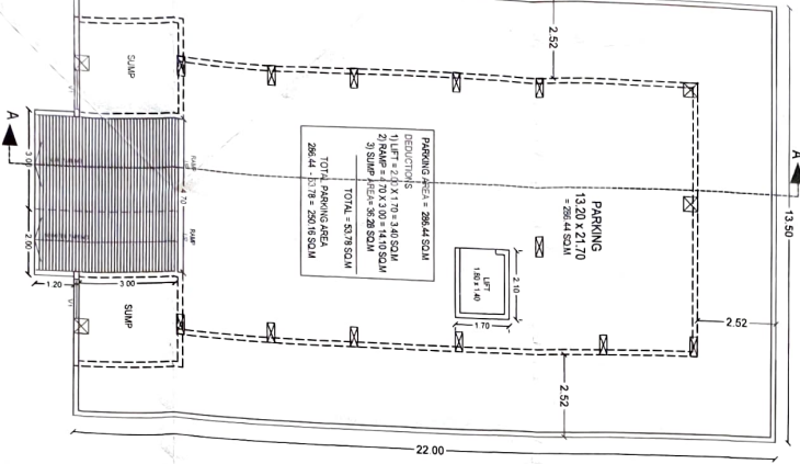
PROPOSED BASEMENT FLOOR PLAN
