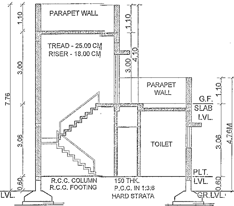
SECTION XX' OF UNIT -A SC:-1:100
