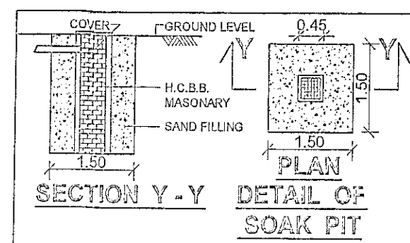
DETAIL OF SOAK PIT
