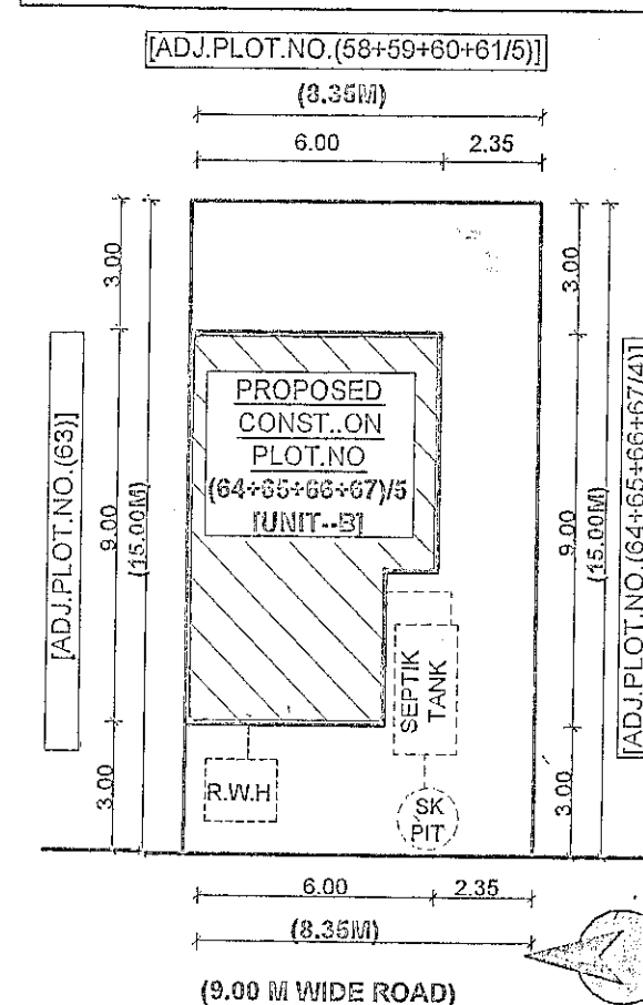
SITE PLAN OF PLOT (64+65+66+67/5) SC:-1:200
