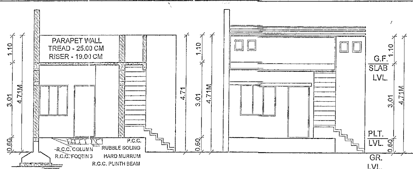
SECTION XX' OF UNIT -A SC:-1:100
