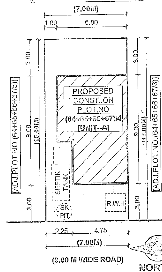
SITE PLAN OF PLOT (64+65+66+67/4) SC:-1:200
