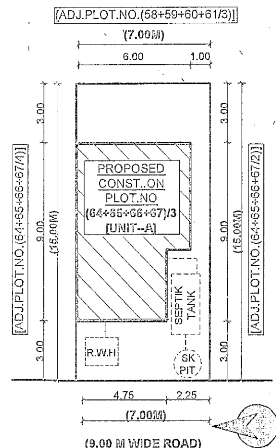
SITE PLAN OF PLOT (64+65+66+67/3) SC:-1:200
