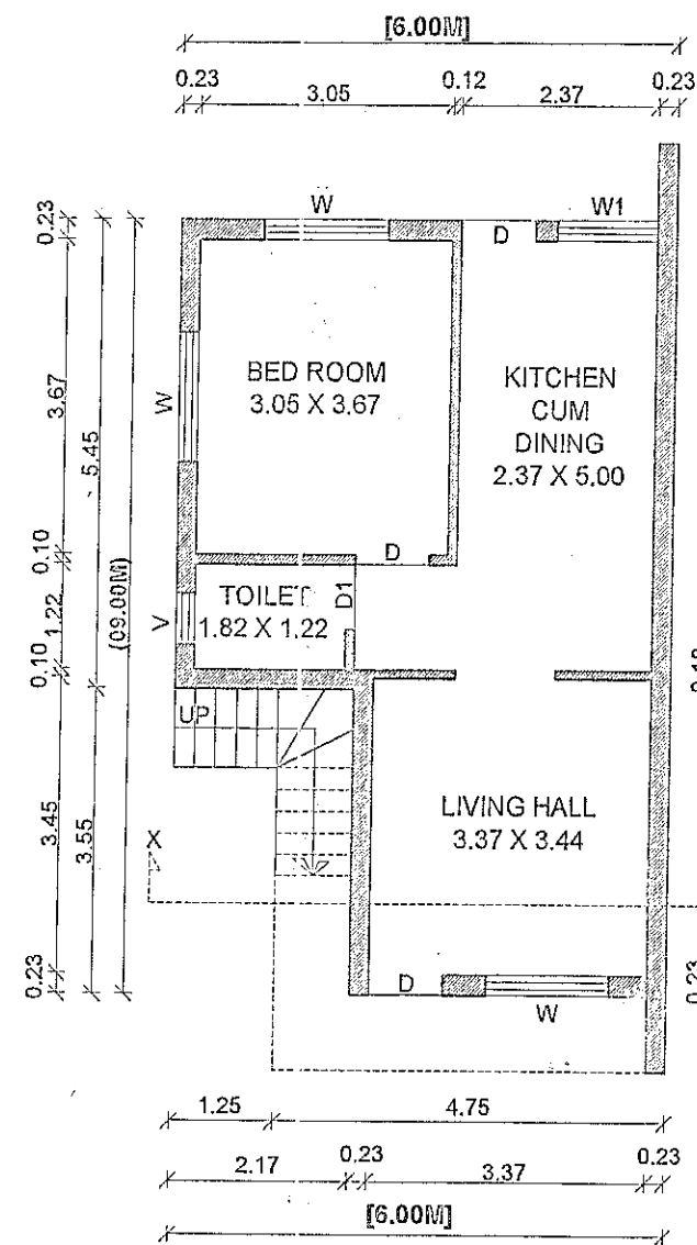
GROUND FLOOR PLAN OF UNIT - (A) (TYPICAL FLOOR PLAN) SC:-1:100
