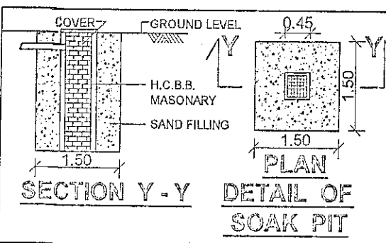
DETAIL OF SOAK PIT
