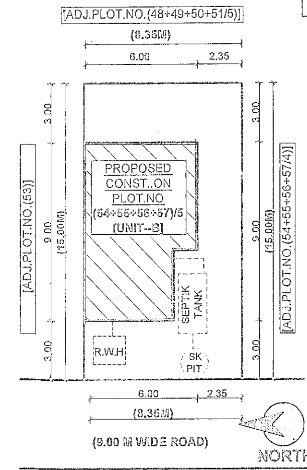
SITE PLAN OF PLOT (54+55+56+57/5) SC:-1:200
