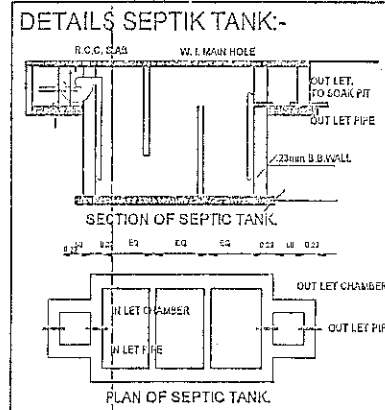
DETAILS SEPTIK TANK:-
