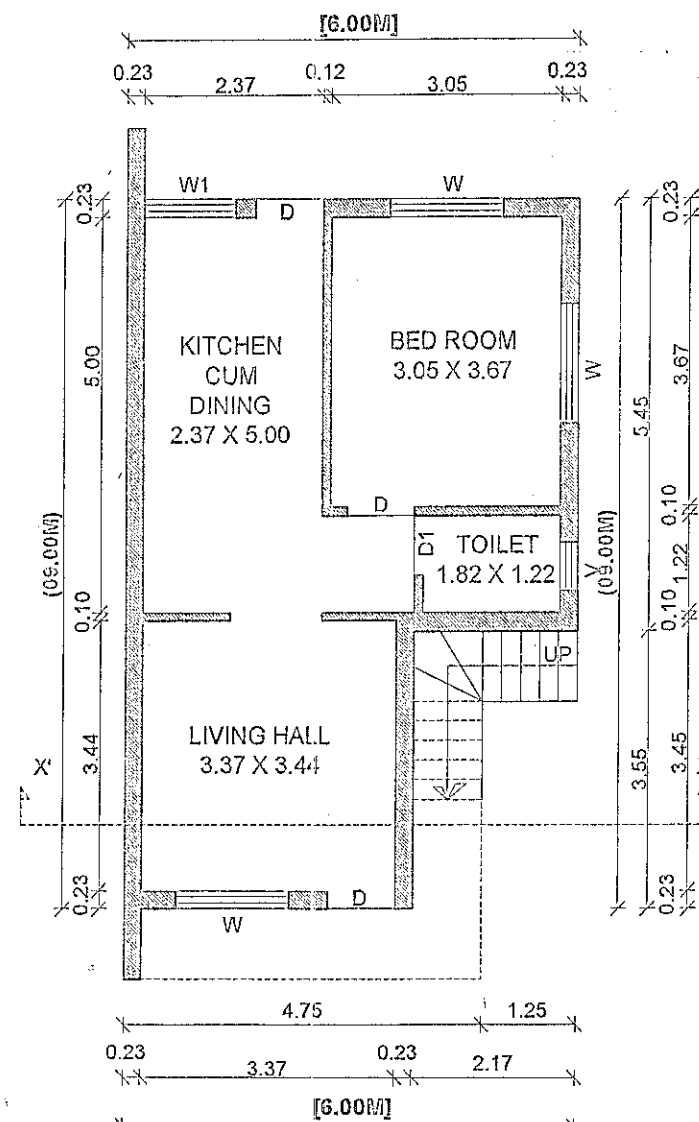
GROUND FLOOR PLAN OF UNIT-(B) (TYPICAL FLOOR PLAN) SC:-1:100
