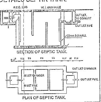
DETAILS SEPTIK TANK-
