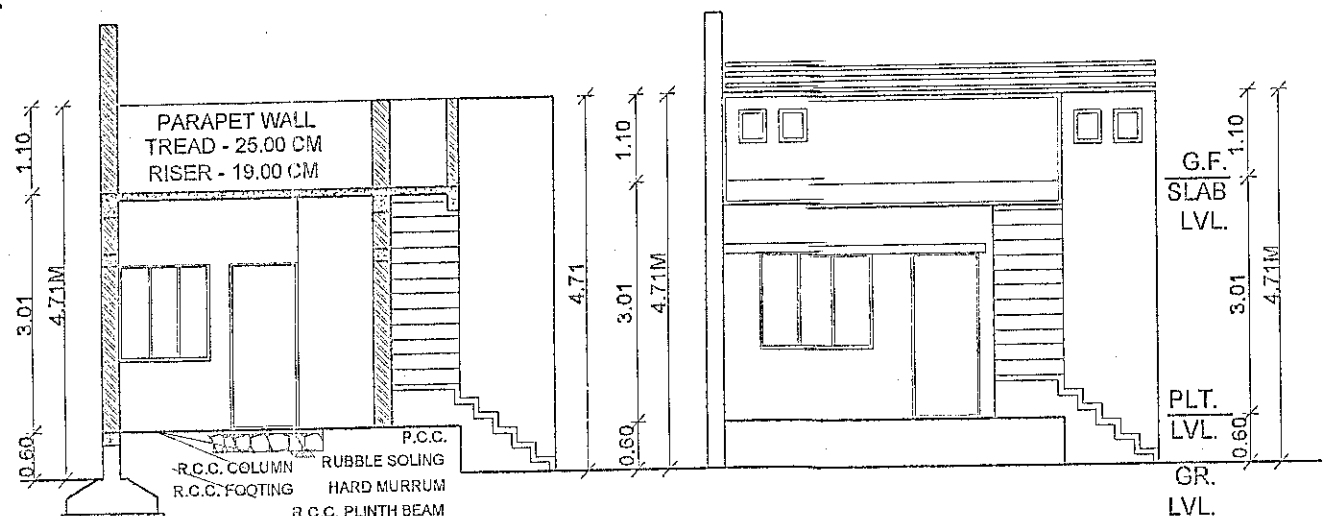
SECTION XX' OF UNIT -A SC:-1:100
