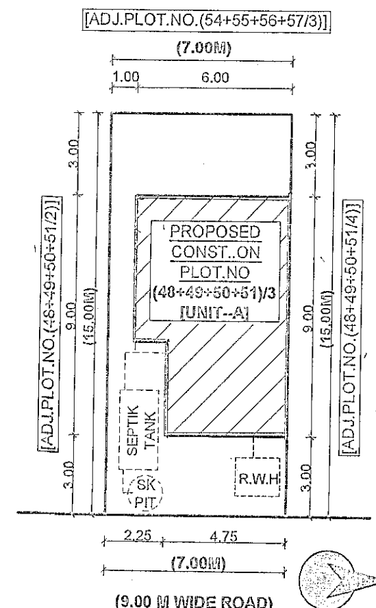
SITE PLAN OF PLOT (48+49+50+51/3)----- SC:-1:200
