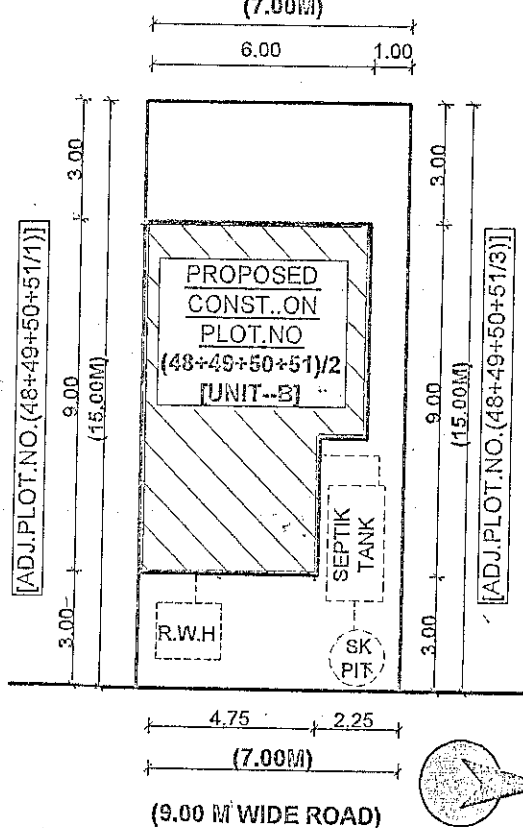
SITE PLAN OF PLOT
