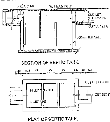
DETAILS SEPTIK TANK-
