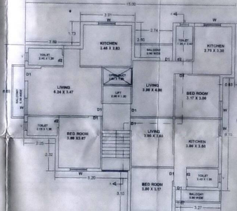
PROP. STILT 1ST & 2ND FLOOR PLAN SCALE: 1:100
