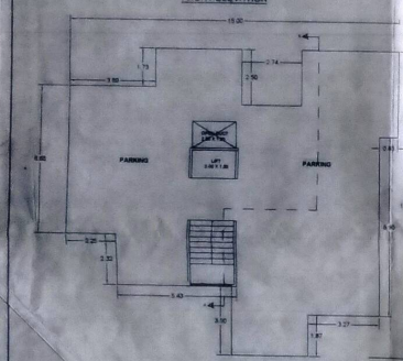
PROP. STILT GR. FLOOR PLAN SCALE: 1:100
